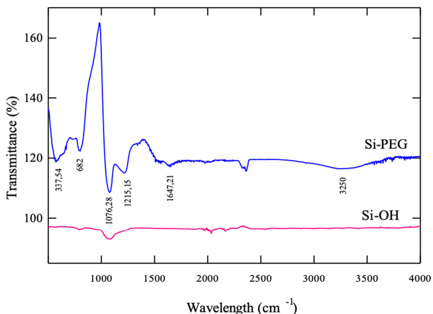
Figure 2. Fourier Transform Infrared (FTIR) spectrum of Si-PEG 4000.
